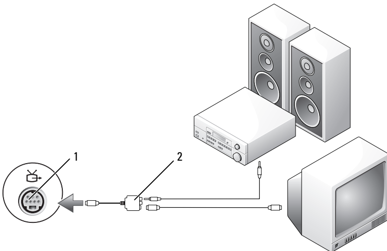
1 S-video TV-out connector 2 composite video adapter
